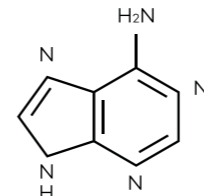
Adenine
