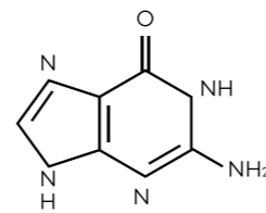
Guanine
